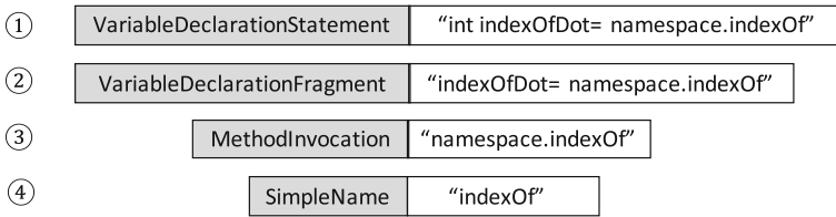
Fig. 9 Excerpt AST of buggy code (Closure-93)
