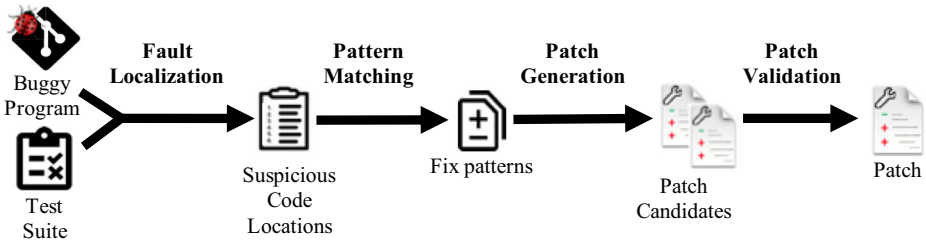
Fig. 16 The overall workflow of PAR FixMiner program repair pipeline
