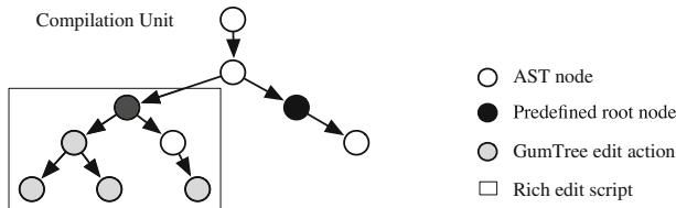
Fig. 8 Illustration of subtree extraction
