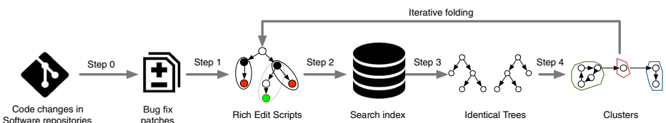
Fig. 5 The FixMiner Approach. At each iteration, the search index is refined, and the computation of tree similarity is specialized in specific AST information details
