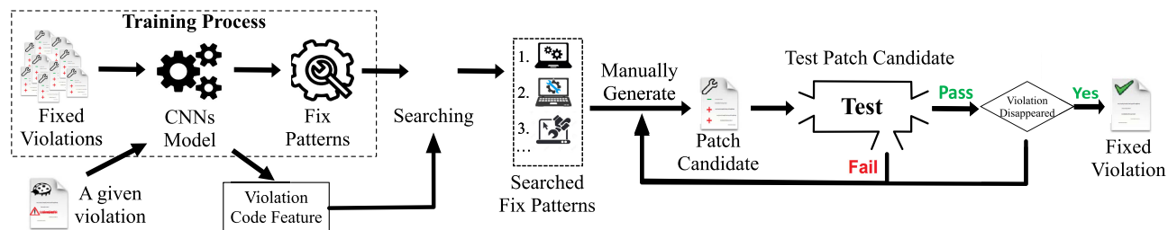
Fig. 19. Overview of fixing similar violations with fix patterns.
